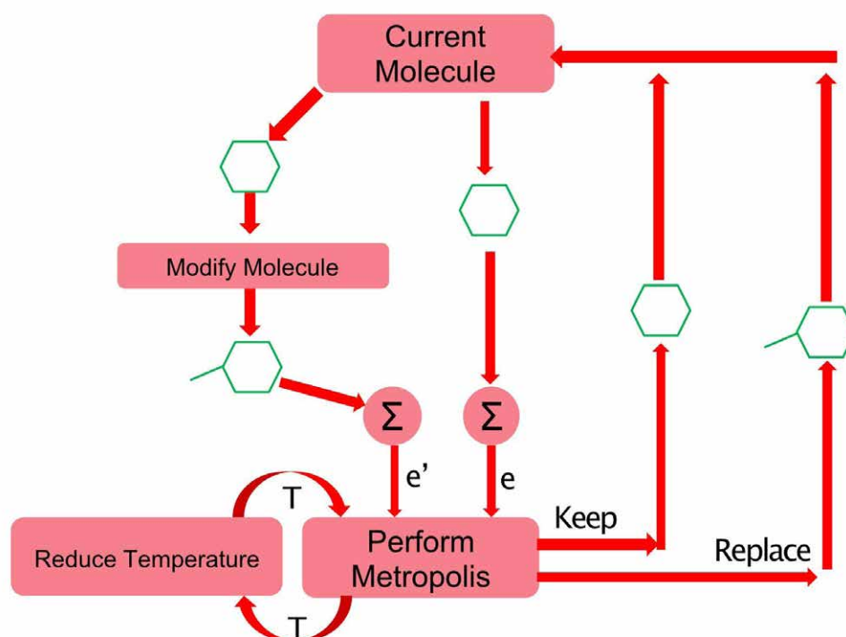
Figure 7: In this illustration of the DA algorithm workflow, random bit vectors (each representing a possible molecule) are used to compute the value of the QUBO. Using a simulated annealing algorithm, executed millions of times in parallel, progressively better molecules are designed.
