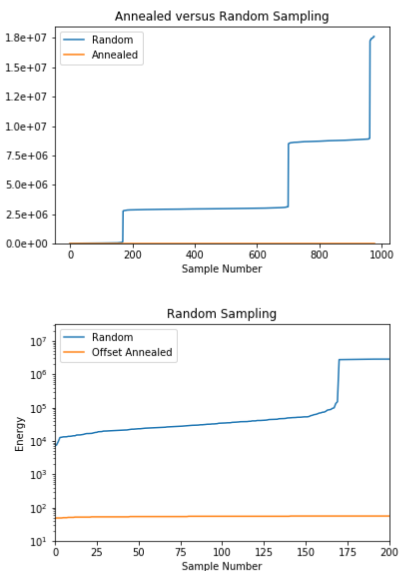
Figure 8: Graphs show the QUBO energies of 1000 random and annealed samples from the chemical space. The lower plot is a zoom in on the lower left corner, plotted using a log scale. [Note that the annealed energy is actually negative, so has been offset by 100 to facilitate display.] It is important to note that none of the random samples reach an energy value of zero, which indicates that the drug-like property constraints are satisfied.
