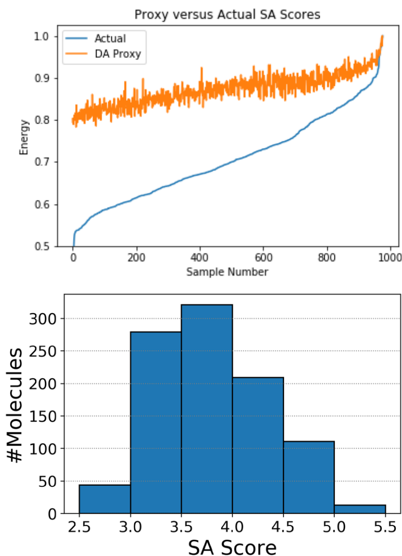
Figure 9: Correlation (top) between actual Synthetic Accessibility (SA) scores and the proxy scores used by the DA. The data are normalized in the range of 0-1, for clarity. Distribution (bottom) of actual SA scores of the designed 977 molecules as calculated from the scripts written by (Ertl and Schuffenhauer 2009) [14] . Scores below 6 indicate easy synthesizability.
