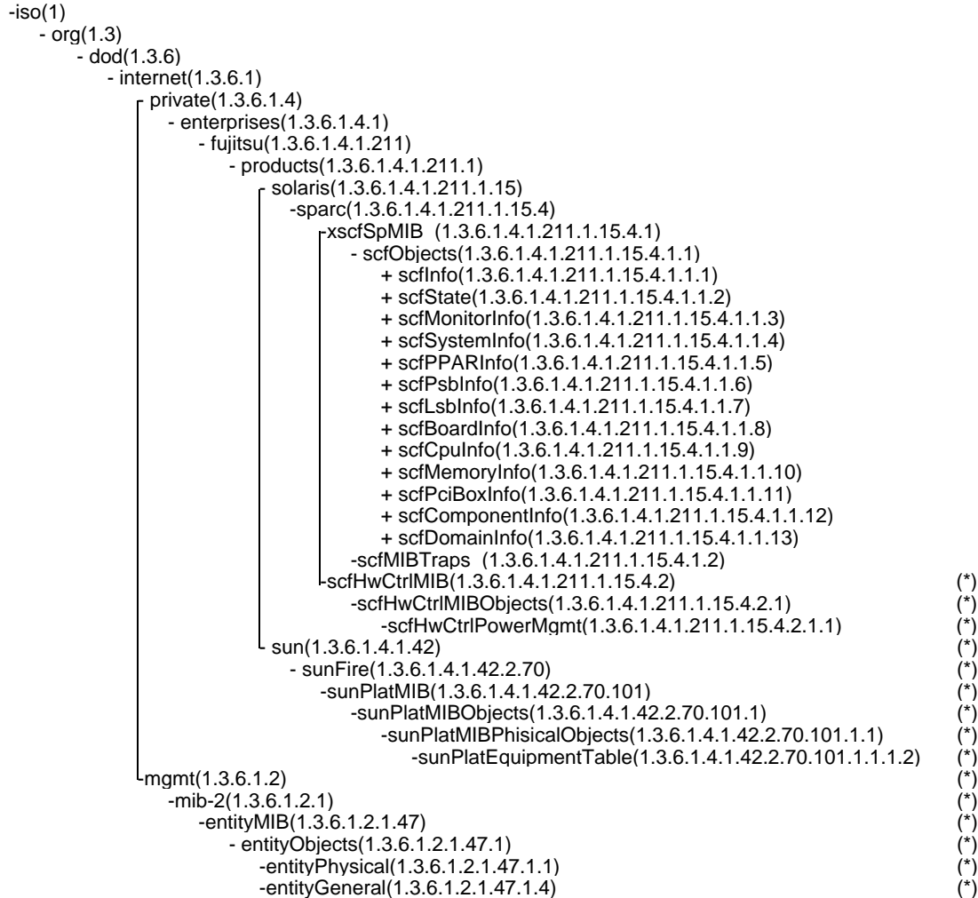
Figure 1-1 MIB tree
