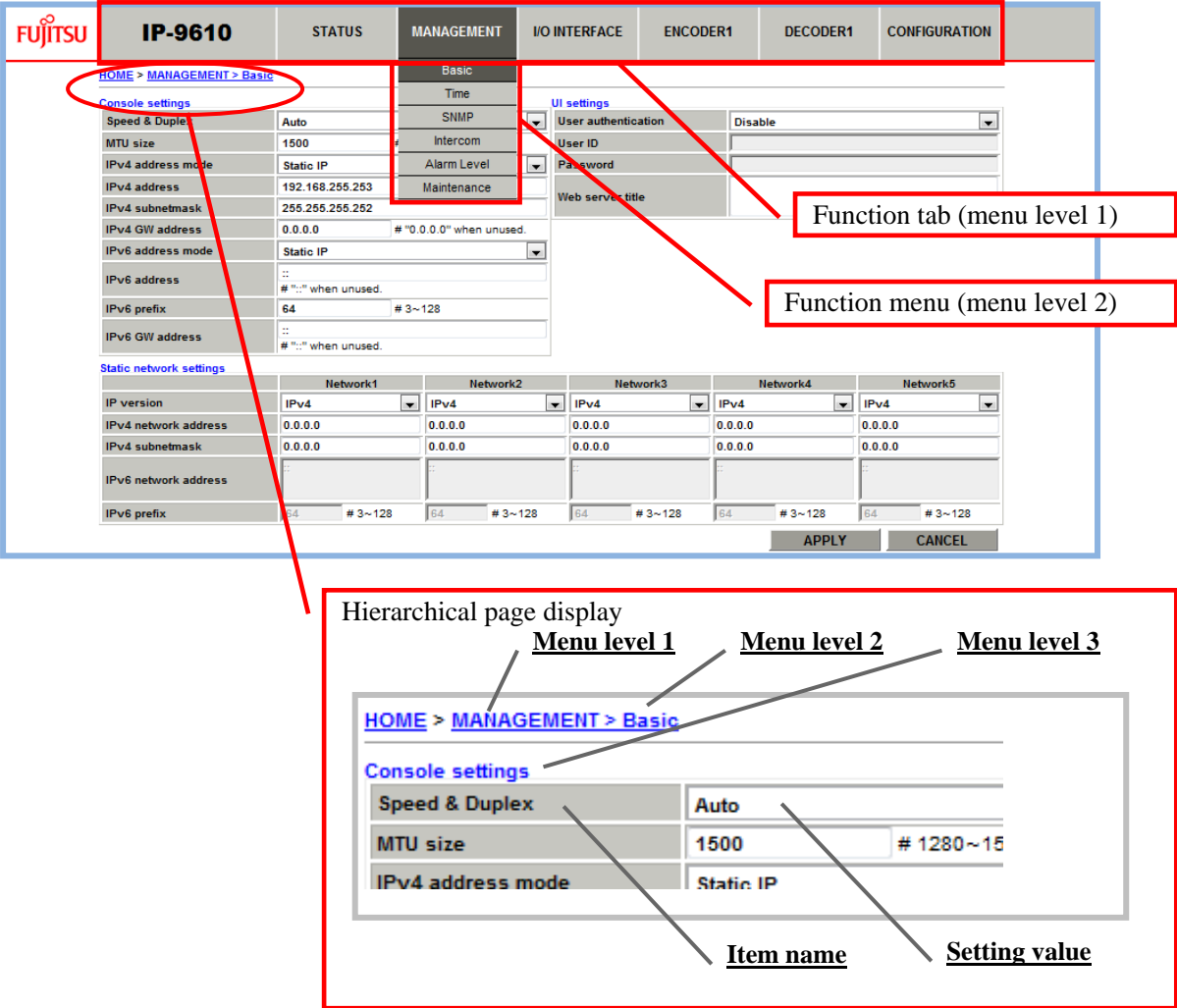
Figure 3.2 IP-9610 Web GUI structure
