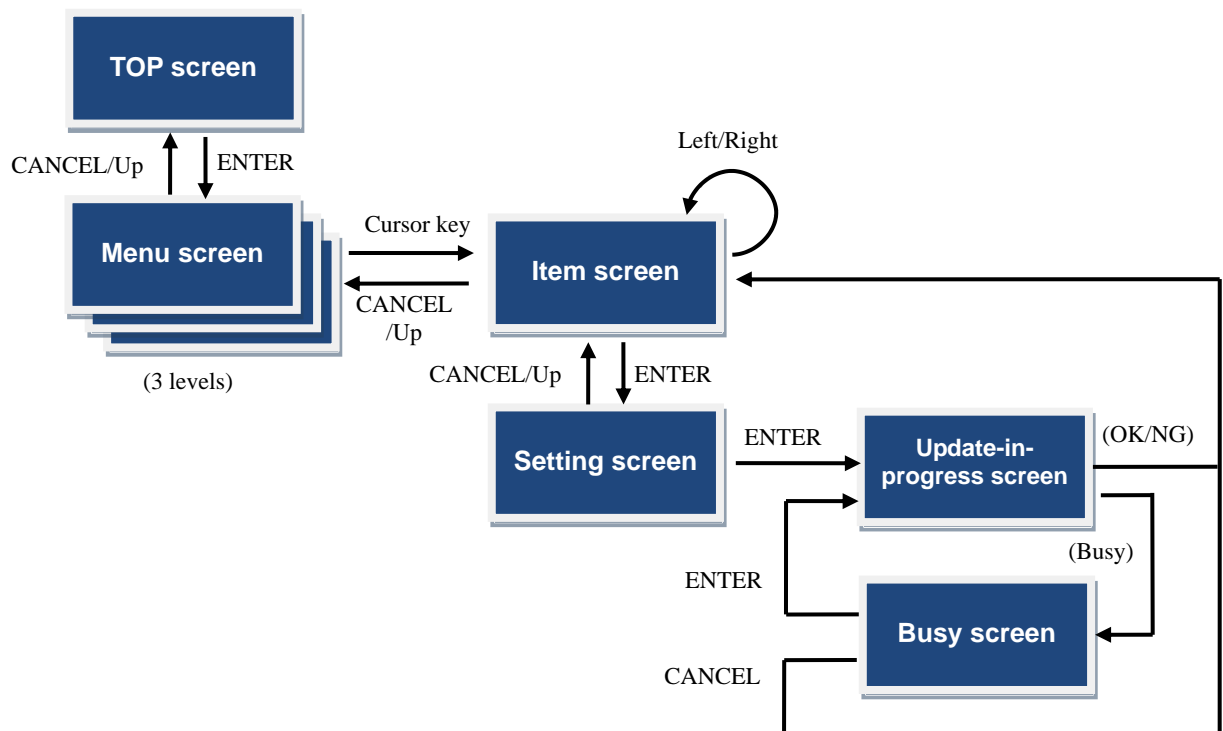
Figure 4-5 Screen transitions on the front panel
