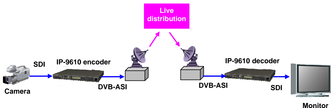
Figure 1.2 e.g. SNG System configuration
