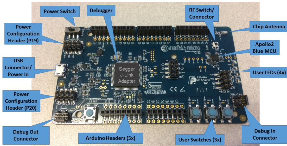
Figure 1. Apollo2 Blue EVB, Revision 0.3
