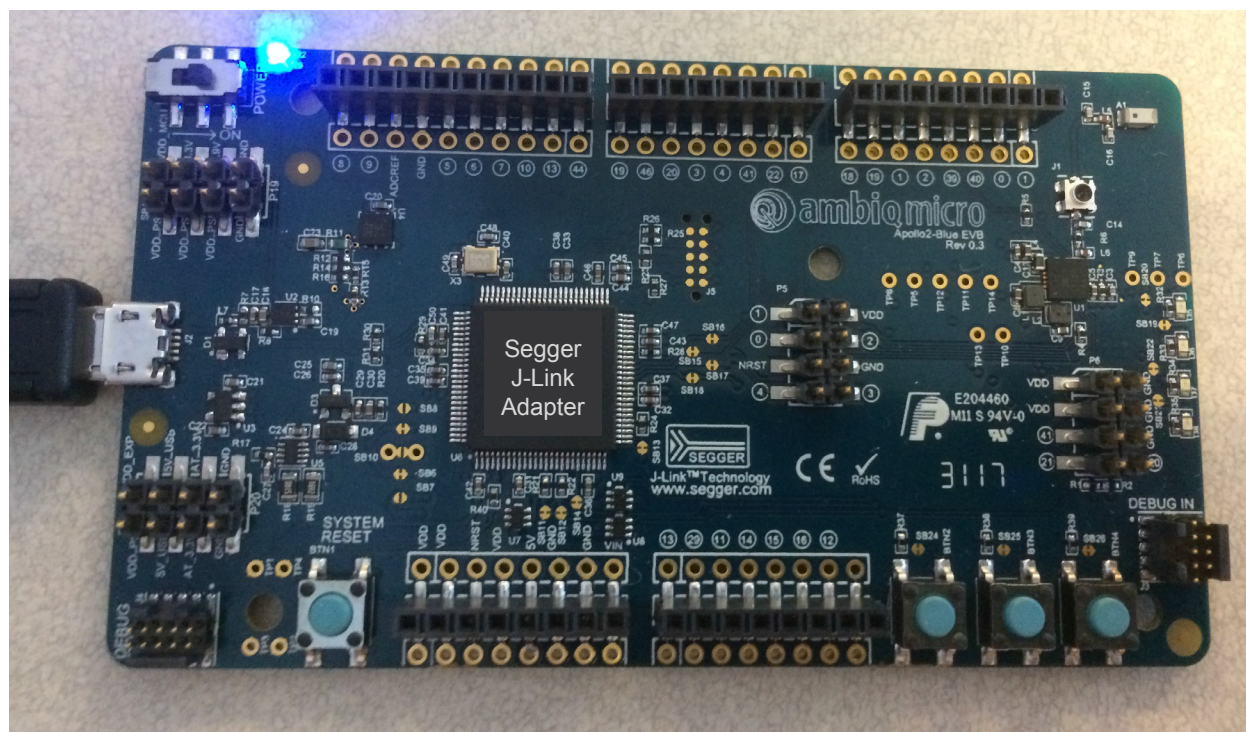
Figure 3. Apollo2 Blue EVB using On-board J-Link Debugger
