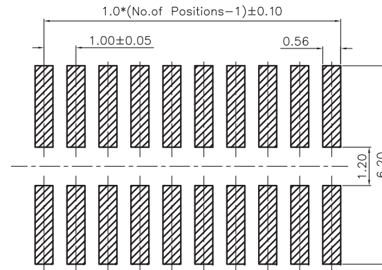
PCB Layout (PCB Tolerance ±0.05)
