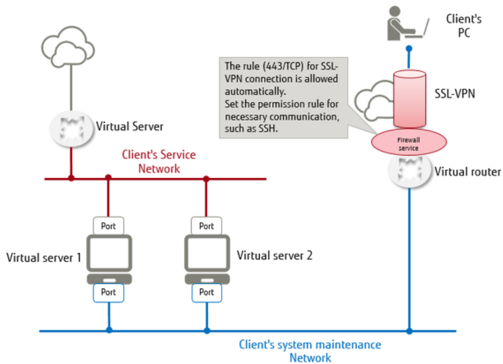
Figure 34: Using SSL-VPN Connection with a Firewall
