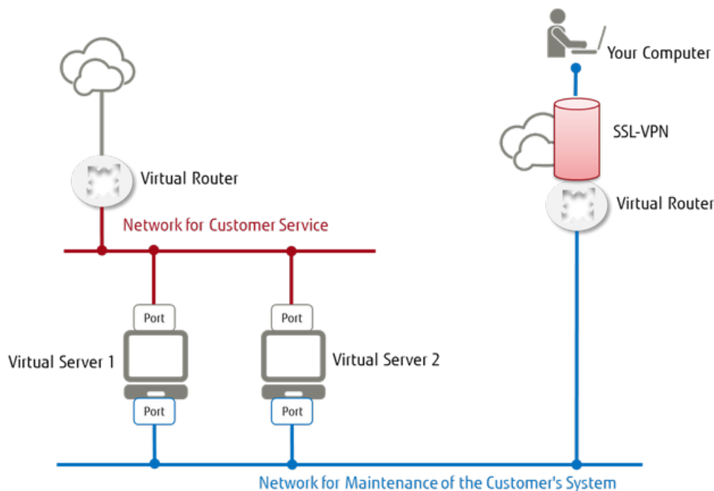
Figure 33: Using SSL-VPN Connection
