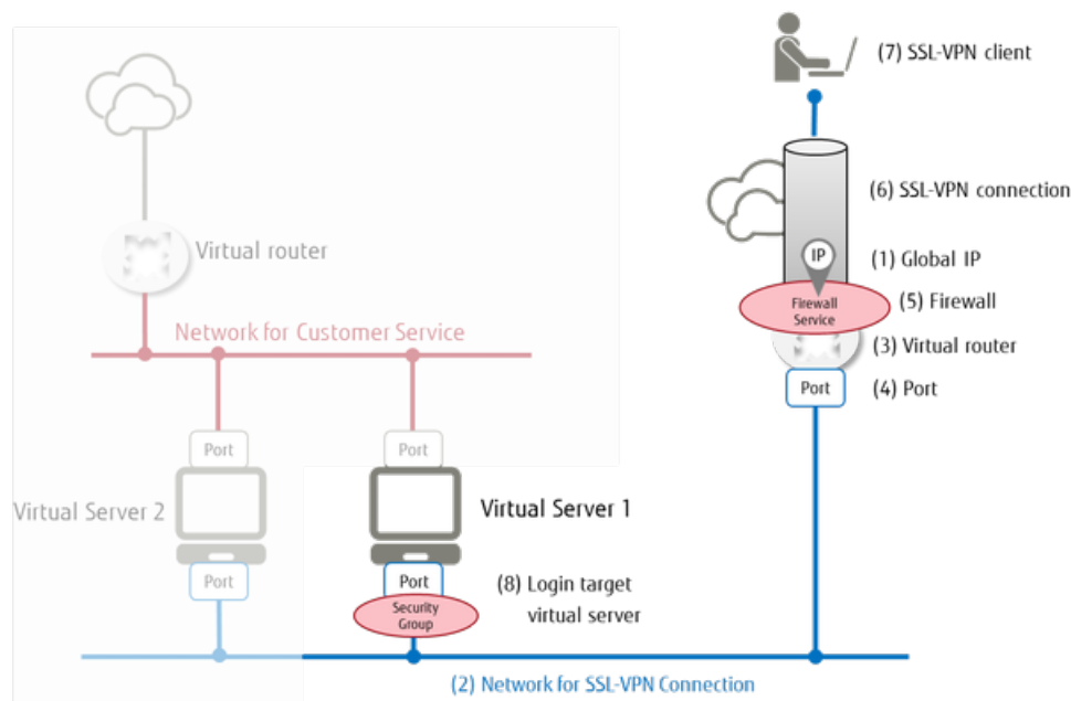
Figure 54: Building an SSL-VPN environment
