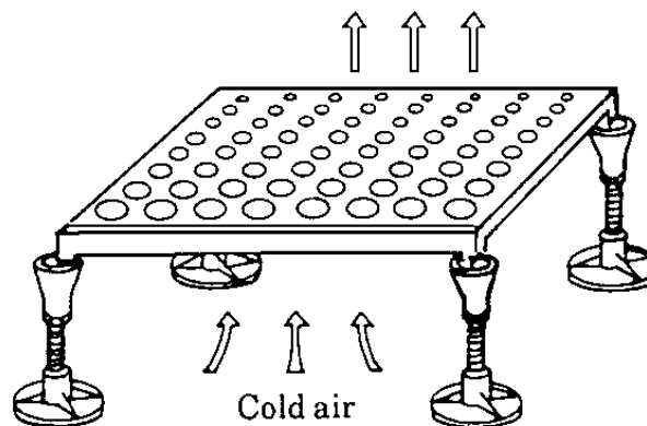
Figure 2.3 Air flow control panel
