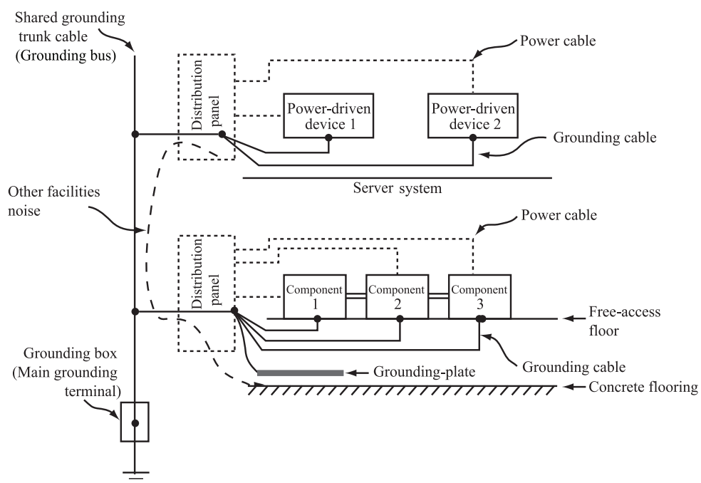
Figure 6.8 Grounding-plate method
