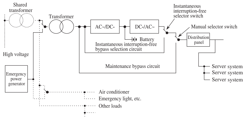
Figure 6.4 System based on a UPS and an independent power generator
