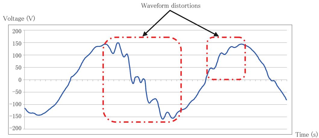
Figure 6.2 AC input voltage waveform (with distortions)
