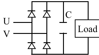
Figure 6.5 Commutating load circuit
