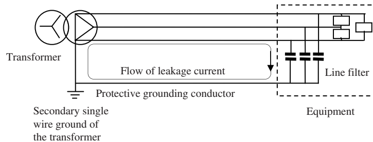
Figure 6.6 Method of grounding equipment
