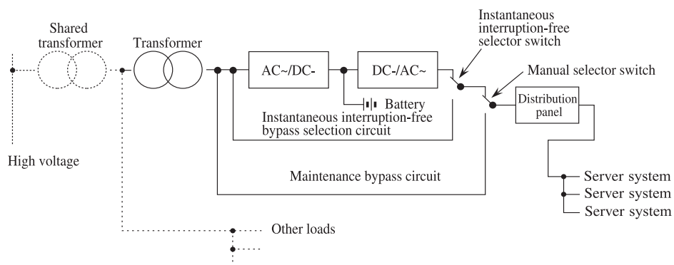
Figure 6.3 System based on a UPS
