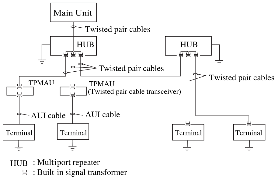
Figure 6.7 Typical 100 Base-T connection
