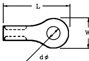
Figure 6.11 Round crimp terminal dimensions
