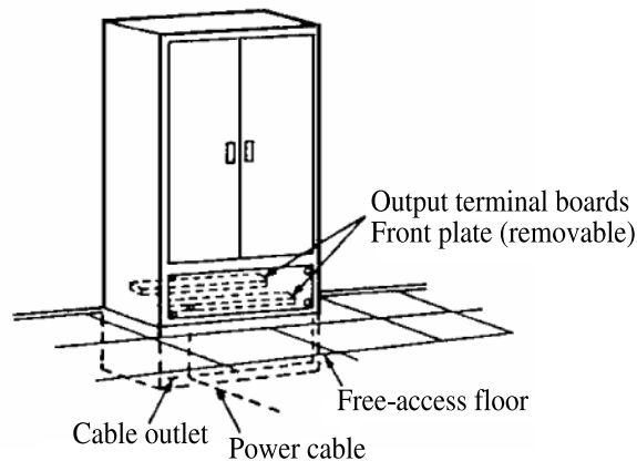
Figure 6.9 Distribution panel (free-standing)
