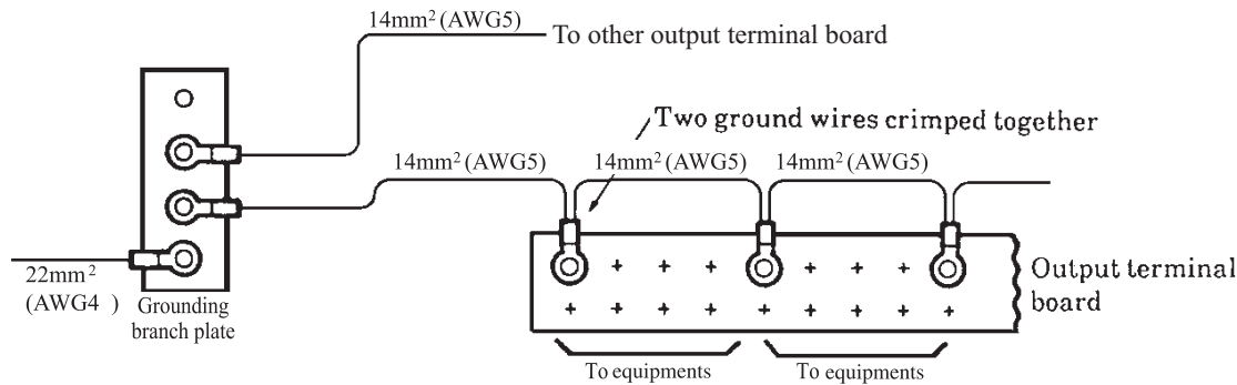
Figure 6.13 Grounding connections within a distribution panel
