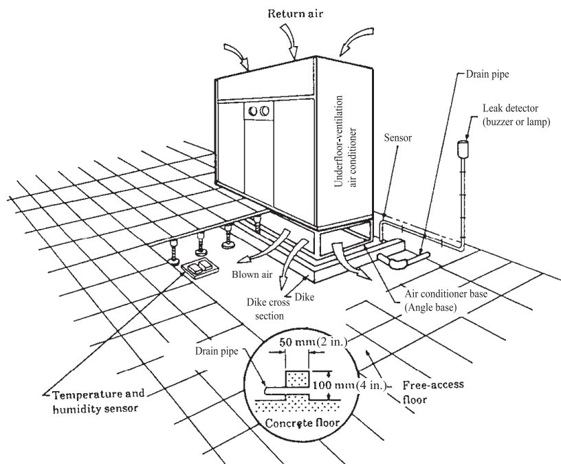
Figure 4.10 Dike
