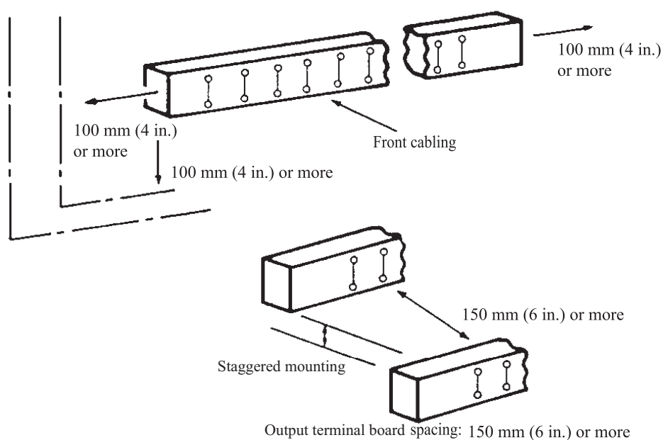
Figure 6.12 Space around output terminal boards
