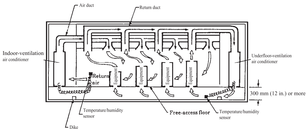
Figure 4.4 Schematic view of a combined system
