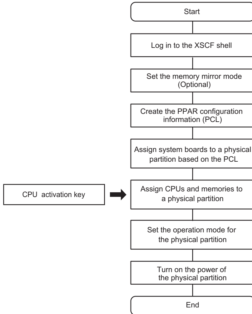
Figure 4-1 Configuring a Physical Partition
