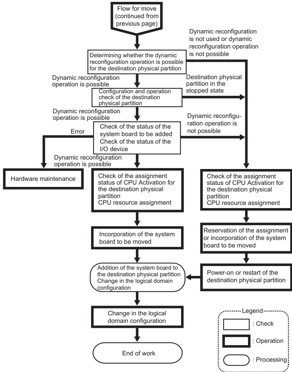
Figure 6-4 Flow for System Board Move (2)
