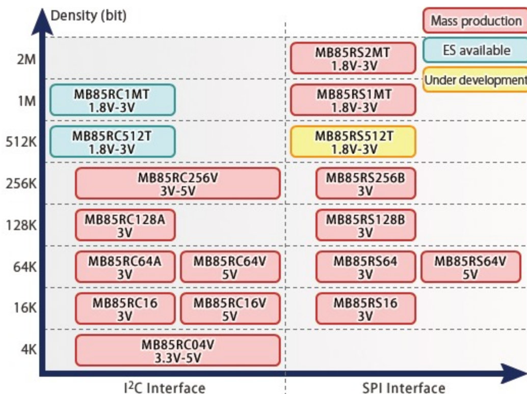
Figure 3: FRAM Product Lineup (Serial Memory)
