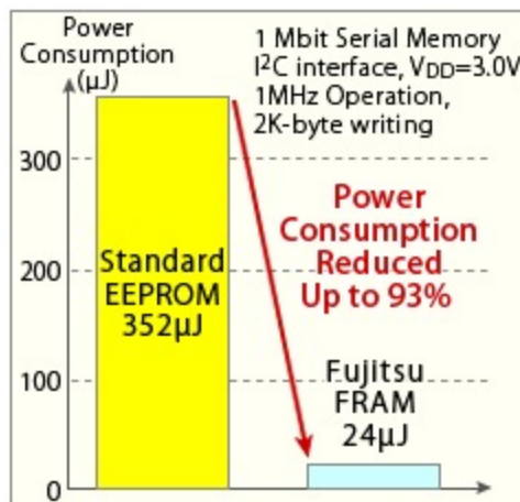
Figure 2: Power Comparison at Writing
