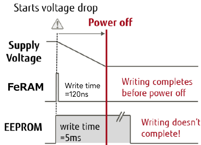
Fig.9: Comparison of Write Time at Power Off
