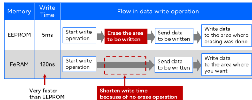
Fig.8: Flow in Data Write Operation
