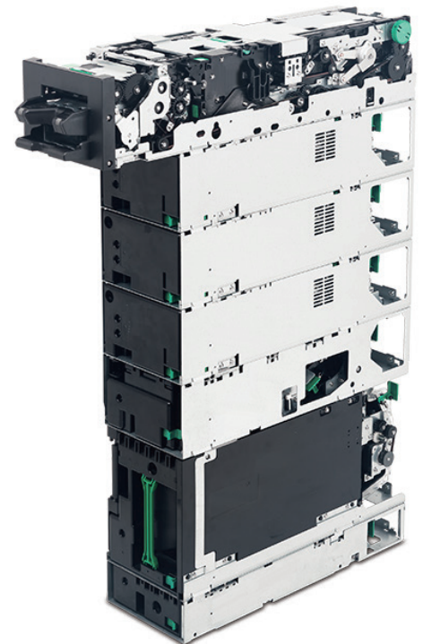
Recycling configuration of GSR50
