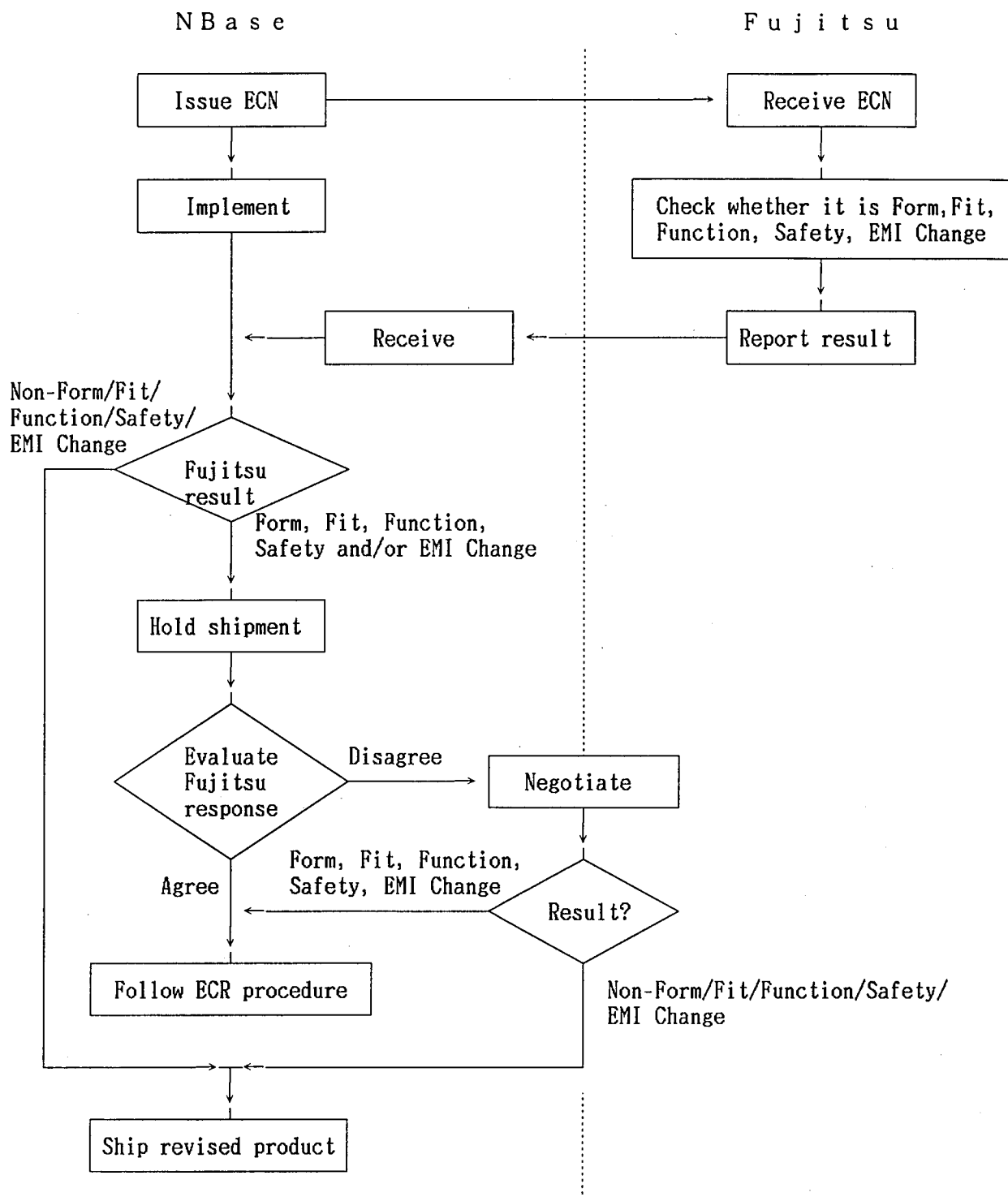
Figure 2 Procedure for Non-Form/Fit/Function/Safety/EMI Change issued by NBase
