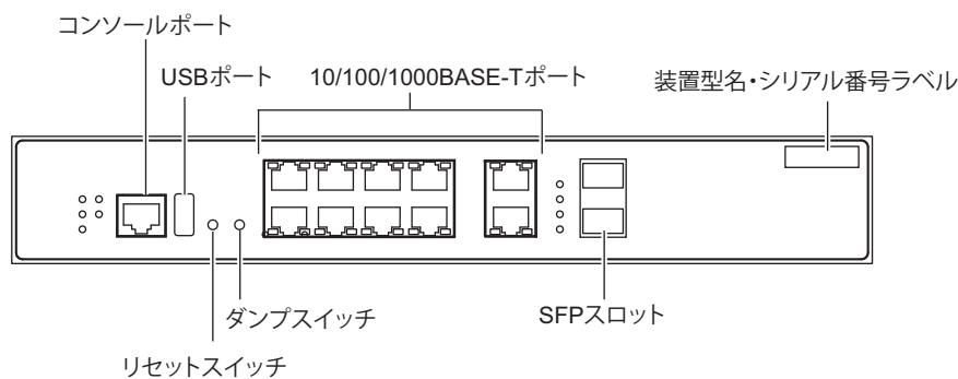
[SR-S318TL2の前面]
