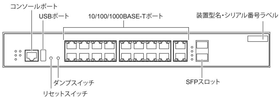
[SR-S318TL2の前面]
