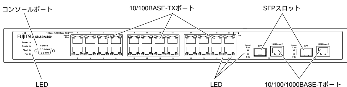
[SR-S224TC2 の前面図]
