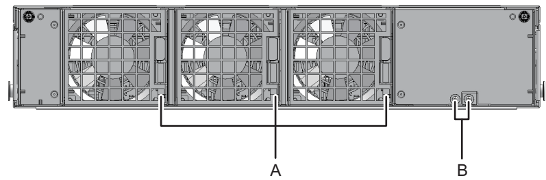
図 2-5 筐体前面のLED
