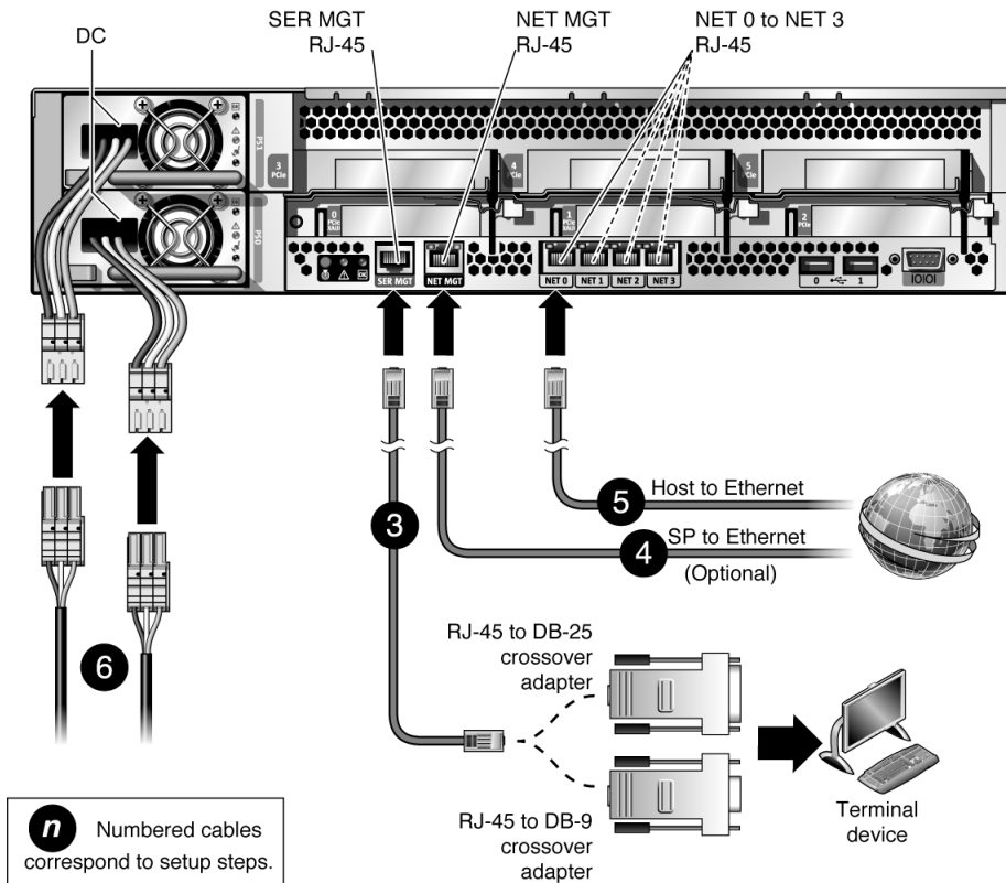
FIGURE 2 Server Connections
