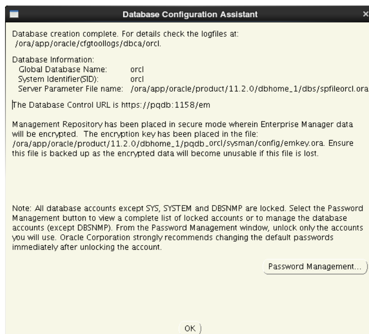
図 4-20 Database Configuration Assistant
