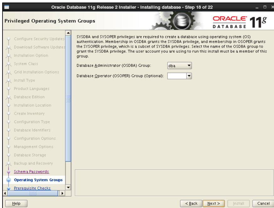
図 4-17 Privileged Operating System Groups
