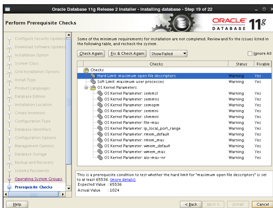
図 4-18 Perform Prerequisite Checks
