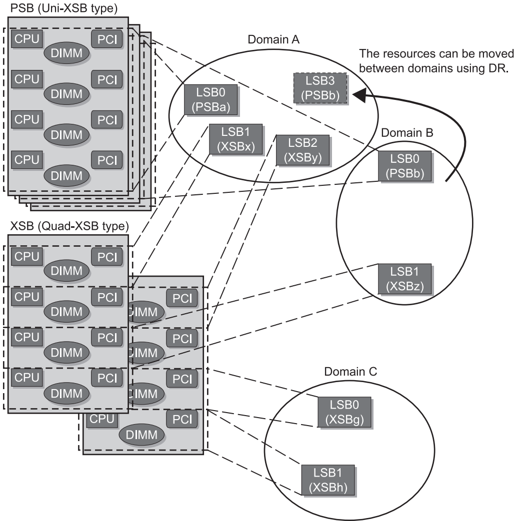
FIGURE 2-4 Domain Configuration
