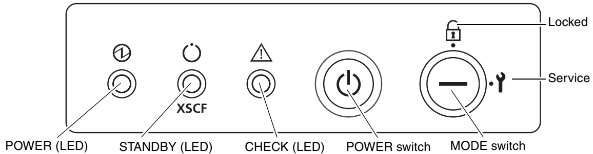
FIGURE 1-10 Operator Panel
