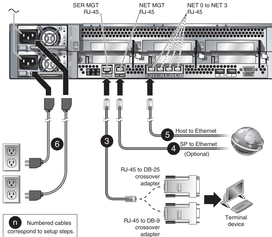
FIGURE 2 Server Connections
