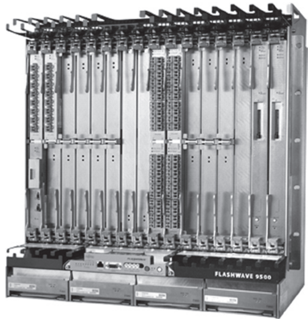
Figure 6 FLASHWAVE 9500 HDS.
