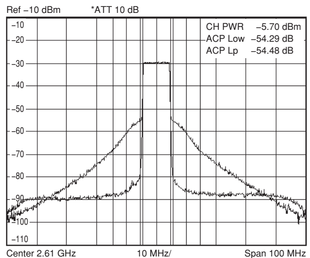
Figure 6 Transmission spectrum.
