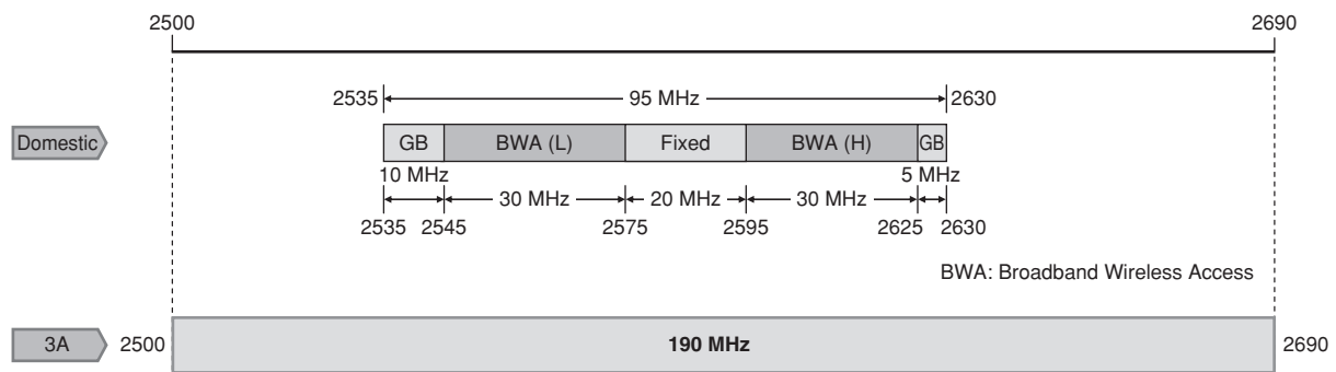
Figure 1 Frequency allocation and coverage of BroadOne WX300 (2.5 GHz Band).
