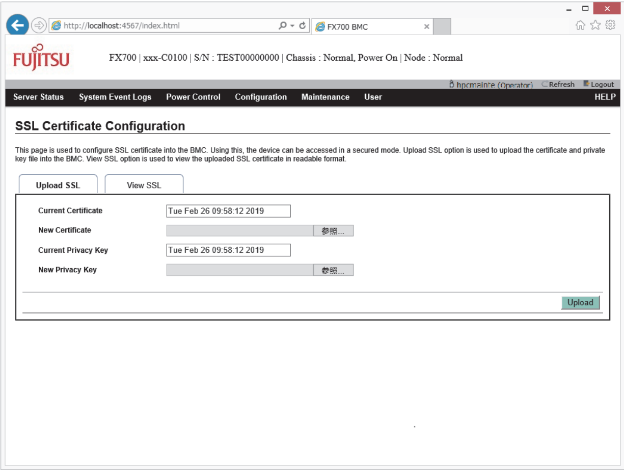
図 3.15 [SSL Certificate Configuration] 画面の [Upload SSL] タブ
