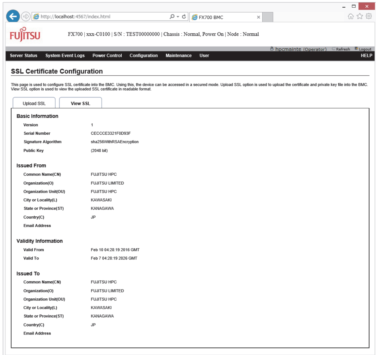
図 3.16 [SSL Certificate Configuration] 画面の [View SSL] タブ
