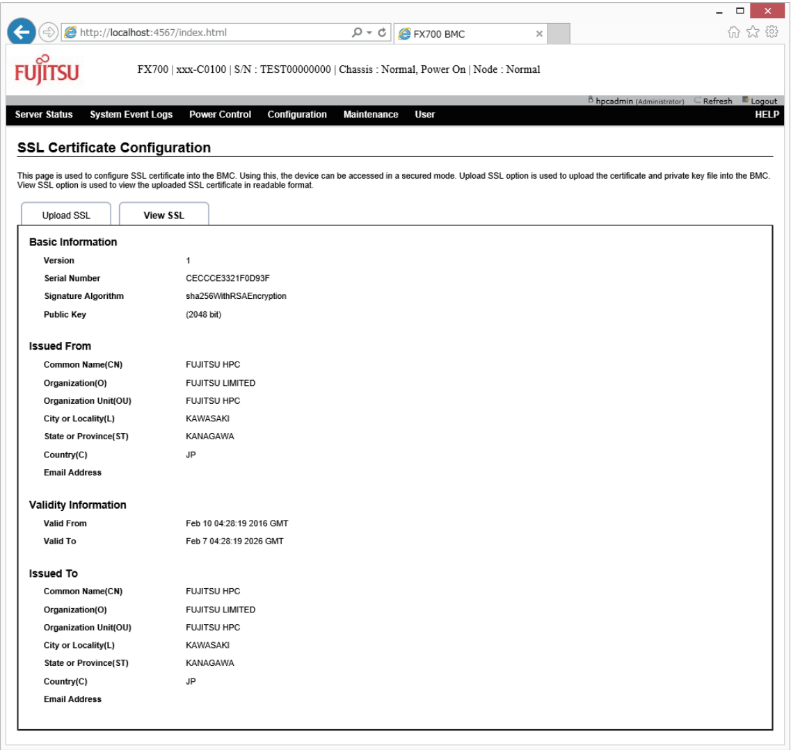
図 3.16 [SSL Certificate Configuration] 画面の [View SSL] タブ
