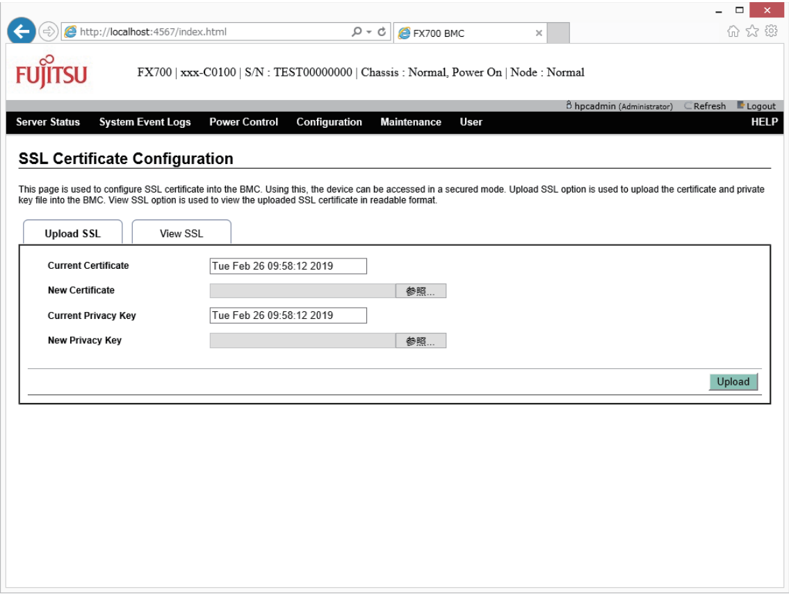
図 3.15 [SSL Certificate Configuration] 画面の [Upload SSL] タブ
