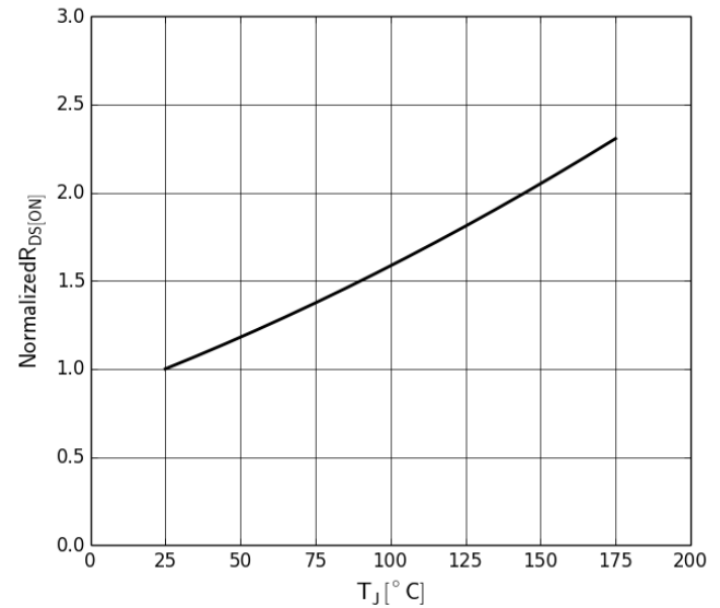
Fig. 4 Normalized On-Resistance I_D=30\text{ A} , V_{GS}=8\text{ V}
