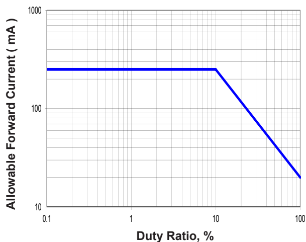
Allowable Forward Current Vs Duty Ratio ( T_a=25 Deg C, t_p \leq 10\mu s )
