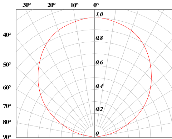
Radiation Pattern
