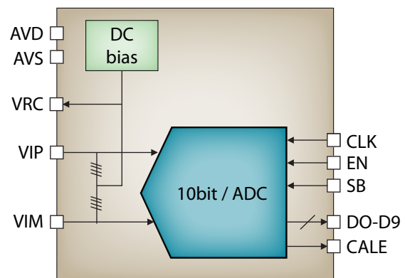
Block diagram
