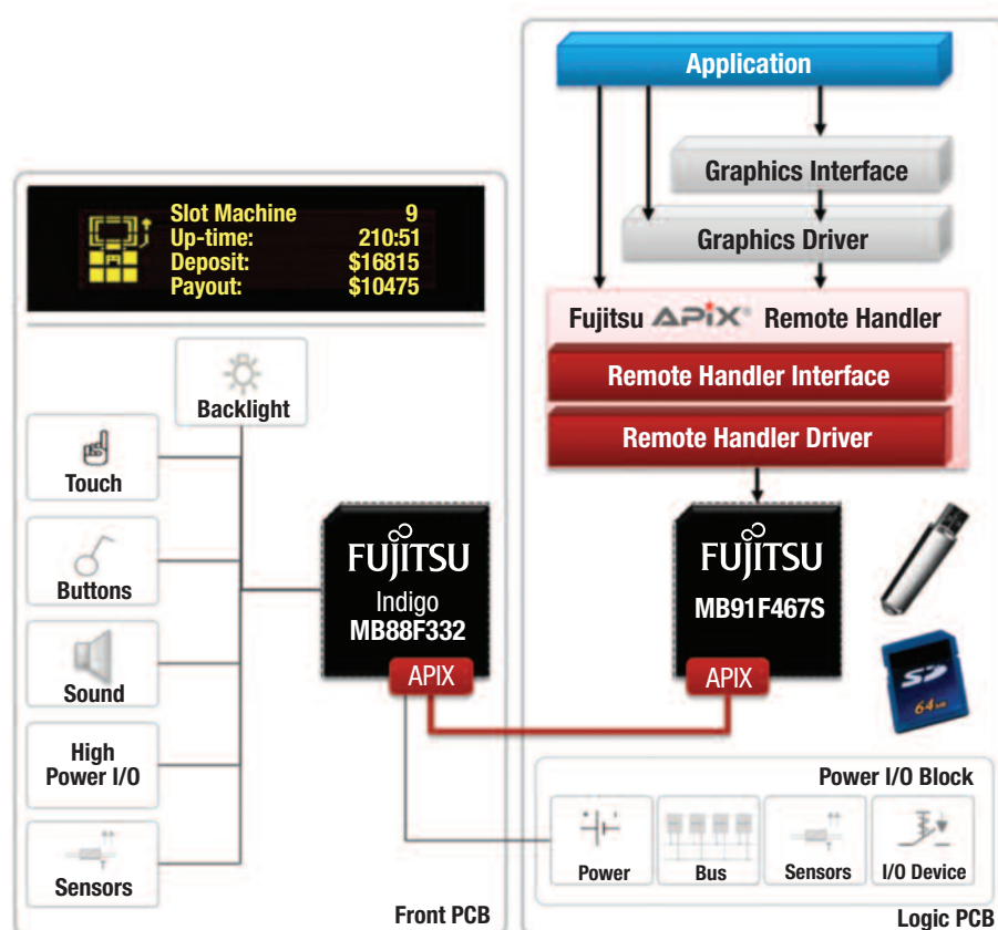
APIX System Block diagram
