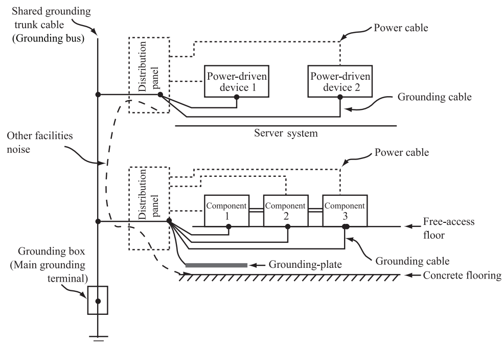
Figure 6.8 Grounding-plate method
