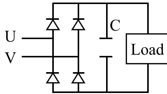
Figure 6.5 Commutating load circuit
