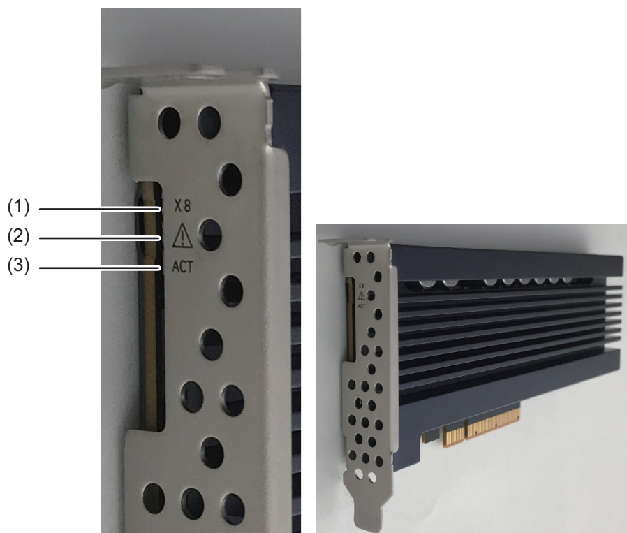
Figure 1-2 Status Indicator LEDs
