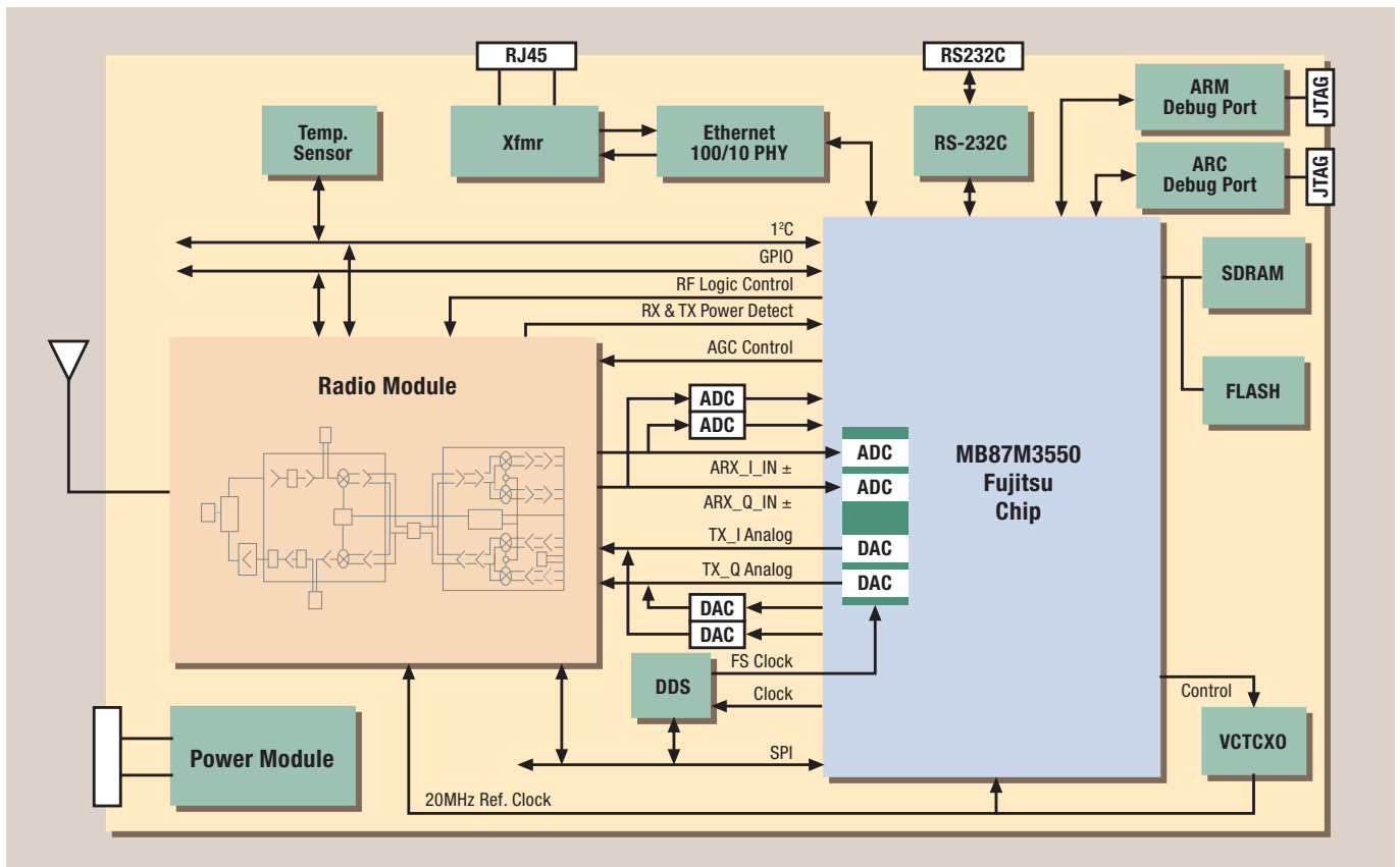
TDD or HDX FDD Reference Board Evaluation System.
