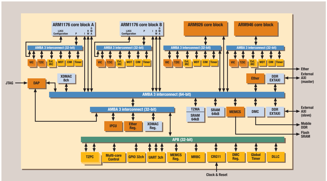
Block diagram of ARM1176 Prototyping Kit.
