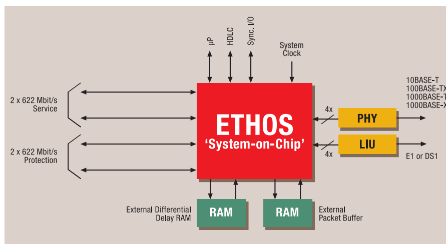
ETHOS used on a slide-in unit in a protected SDH/SONET system.
