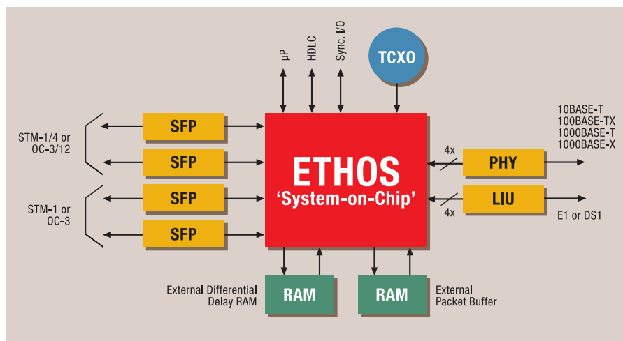
ETHOS used in stand-alone application.
