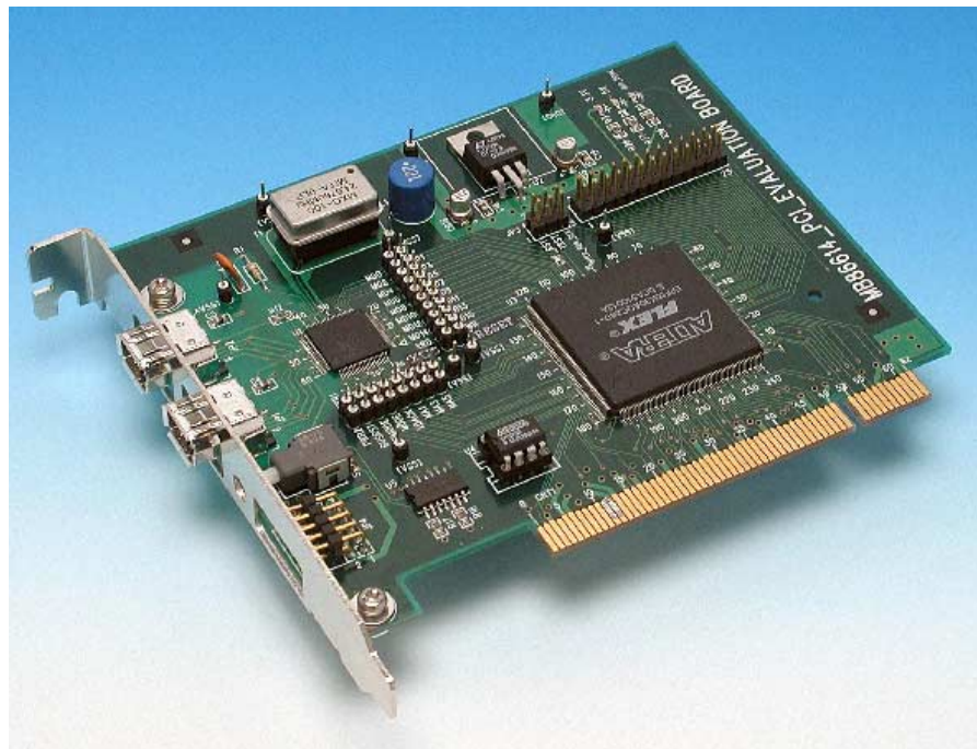
Figure 1: MB86614A PCI Evaluation Board
