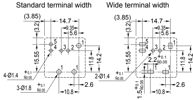
PC board mounting hole layout (BOTTOM VIEW)
