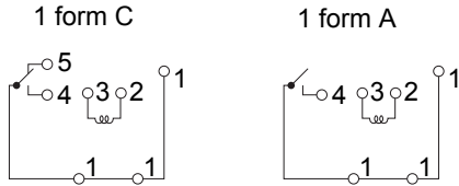
Schematics (BOTTOM VIEW)
