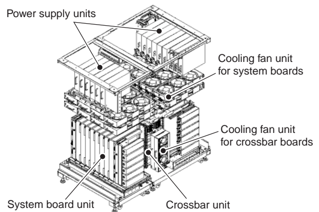
Figure 3 System configuration of PW2500.
