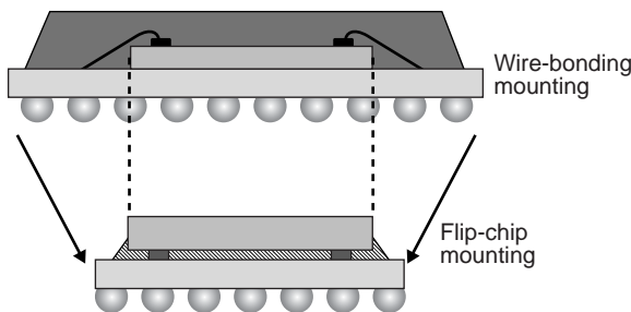
Figure 1 Comparison of wire-bonding and flip-chip mounting.
