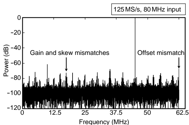
Figure 12 Measured spectrum.
