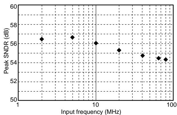
Figure 13 Measured peak SNDR versus input frequency at 125 MS/s.
