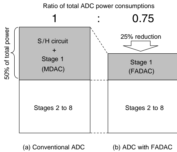
Figure 5 Power reduction achieved using FADAC.
