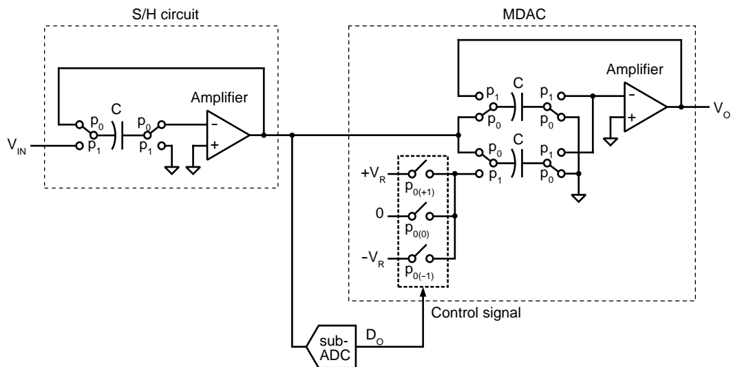
Figure 2 Conventional front-end circuit.
