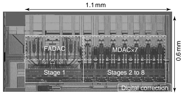
Figure 10 ADC chip photomicrograph.
