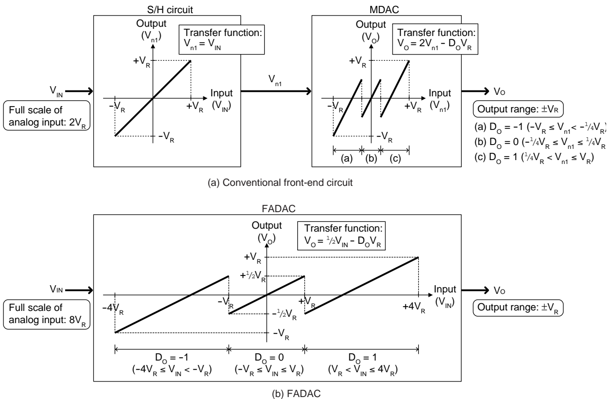
Figure 6 Comparison of transfer functions.
