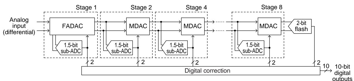
Figure 7 Block diagram of prototype ADC.
