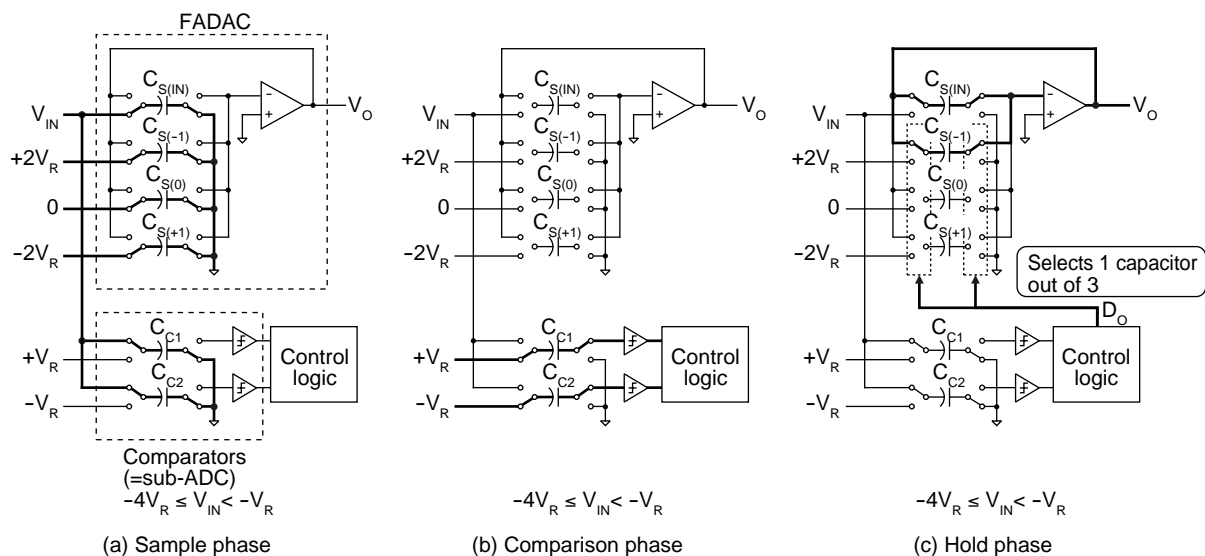
Figure 3 Schematic and operation of flip-around digital-to-analog converter (FADAC).
