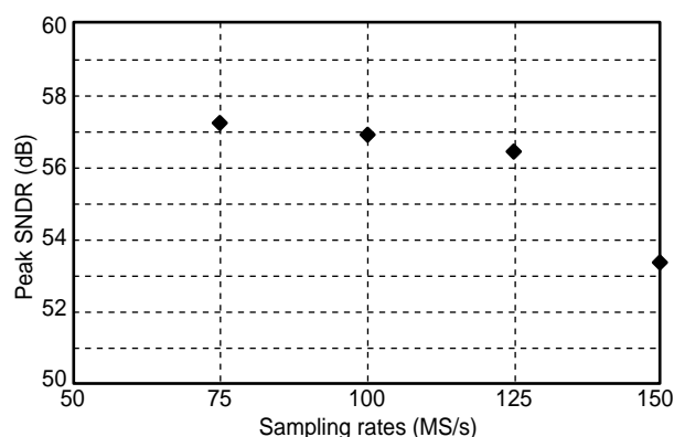
Figure 14 Measured Peak SNDR versus sampling rates at 2 MHz sinusoidal input.
