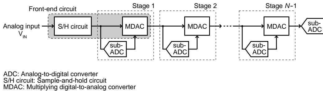
Figure 1 Conventional pipeline architecture.
