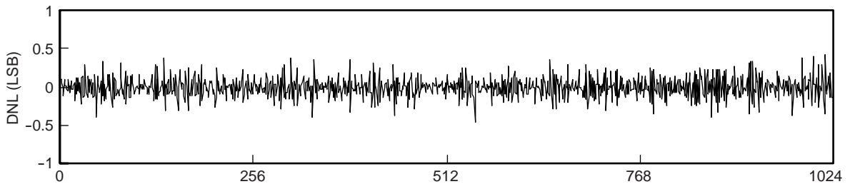
(a) DNL curve
