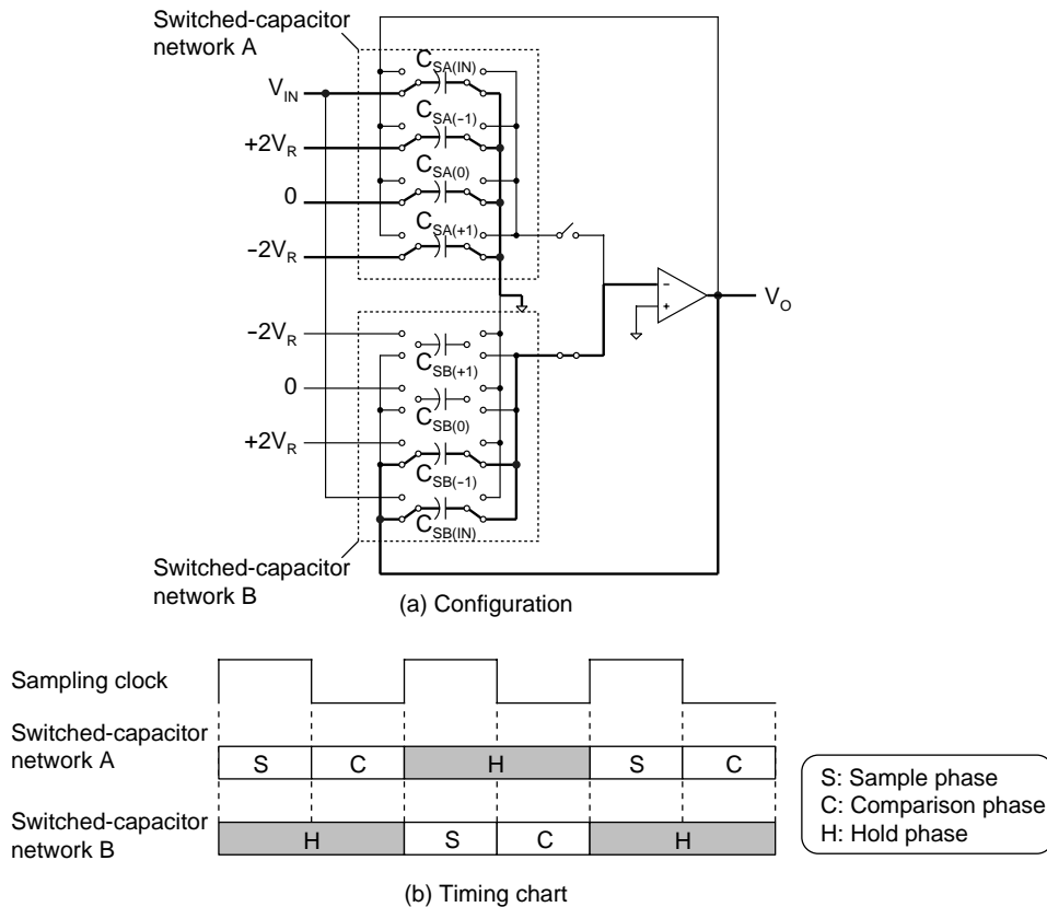
Figure 8 Configuration and timing chart of double-sampling FADAC.
