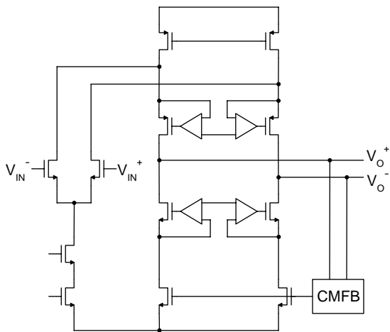
CMFB: Common-mode feedback circuit
