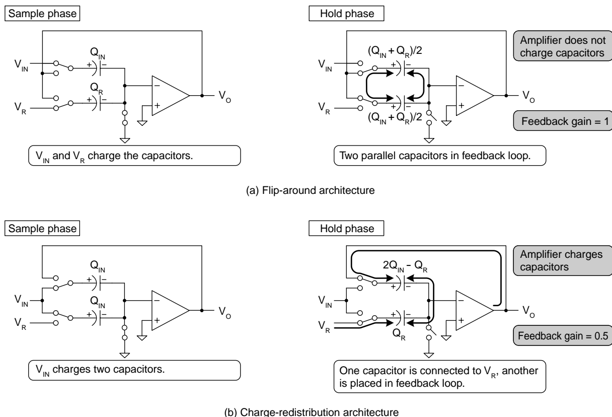
Figure 4 Comparison of flip-around and charge-redistribution architectures.
