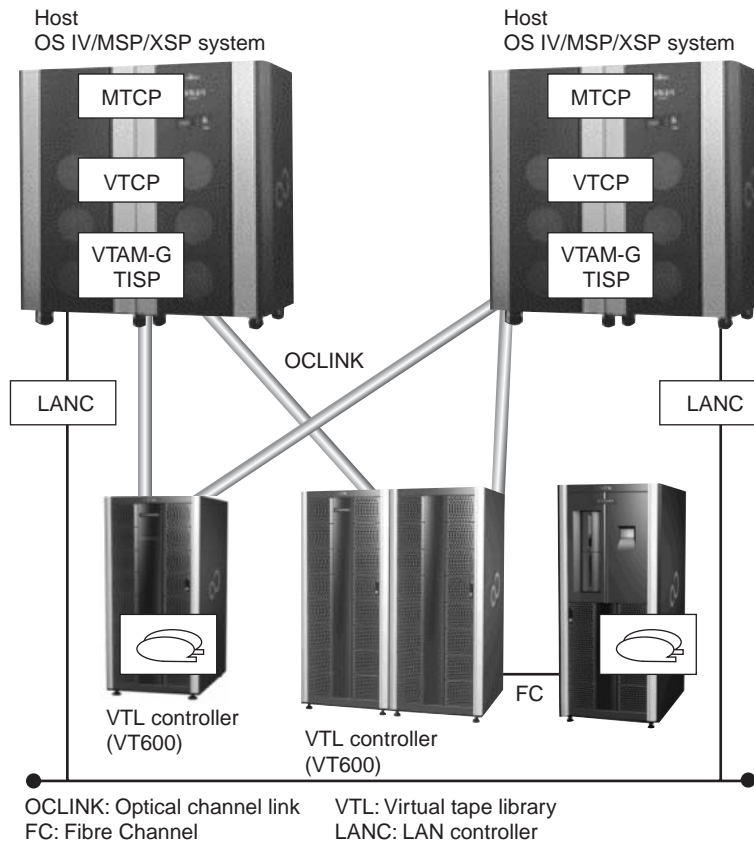
Figure 2 System configuration.
