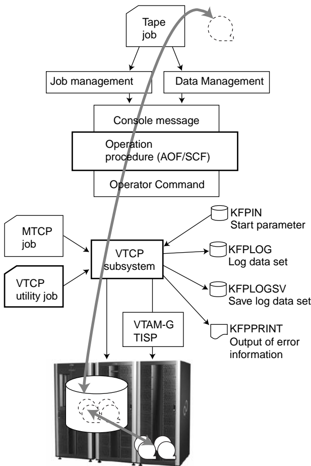
Figure 8 VTCP operation.
