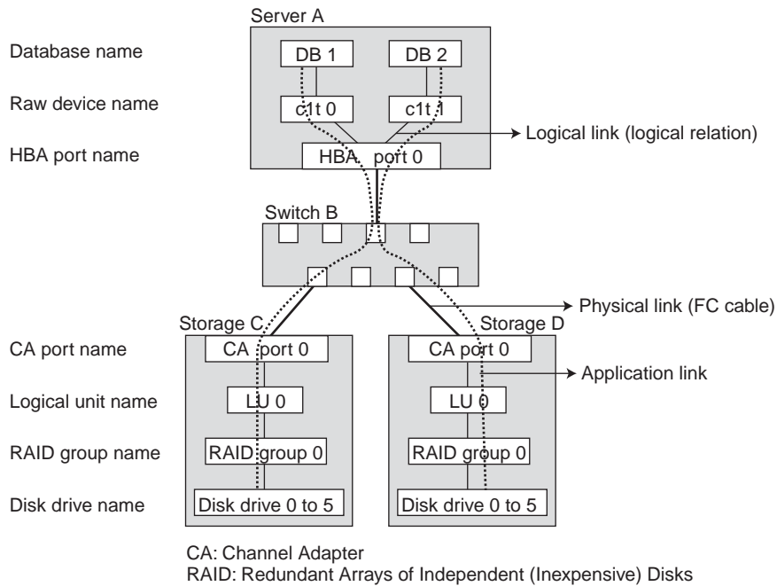
Figure 2 Logical/physical/application links.
