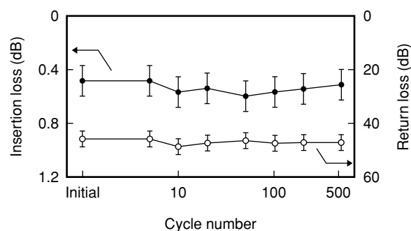
Figure 13 Insertion and return losses of Type I array in temperature cycle test.
