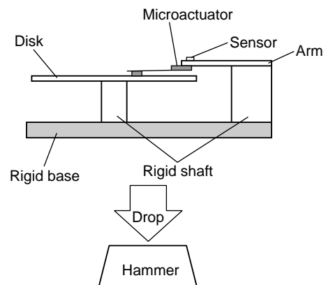
Figure 5 Impact tester.
