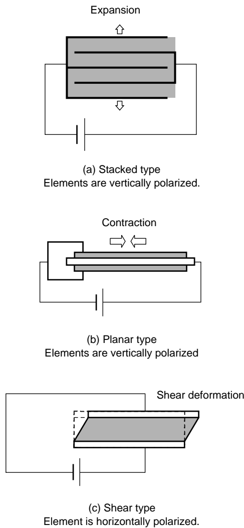
Figure 1 Piezoelectric actuators.
