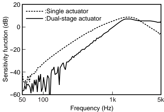
Figure 8 Sensitivity function.
