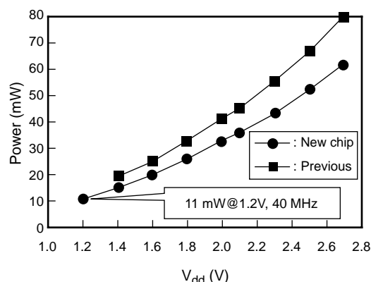
Figure 7 Power consumption.
