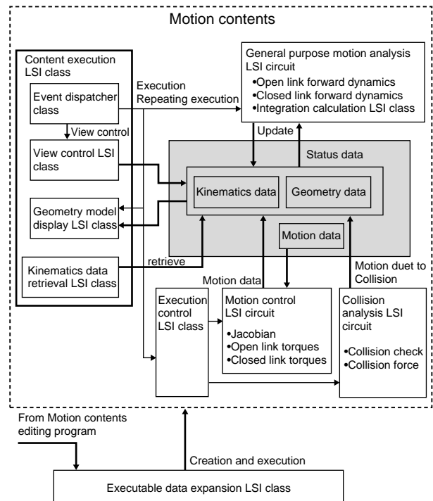
Figure 6 Motion contents execution program.
