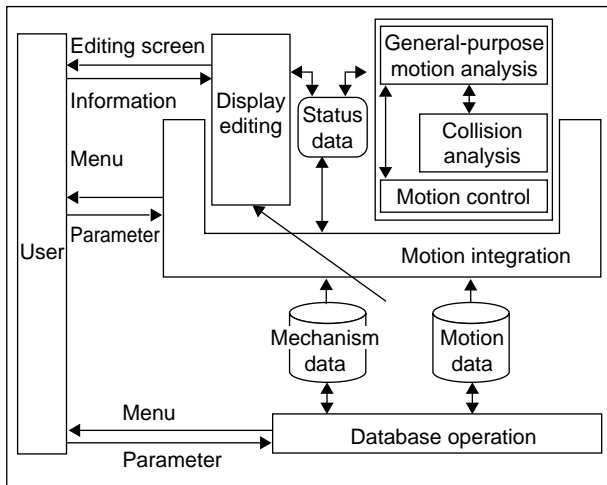
Figure 4 Relations between functions.
