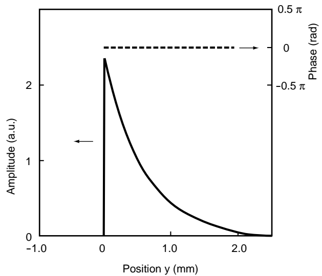
Figure 7 Output beam profile with uniform reflectivity.
