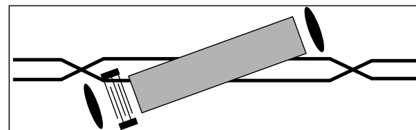
Figure 4 Apodized SAWG.
