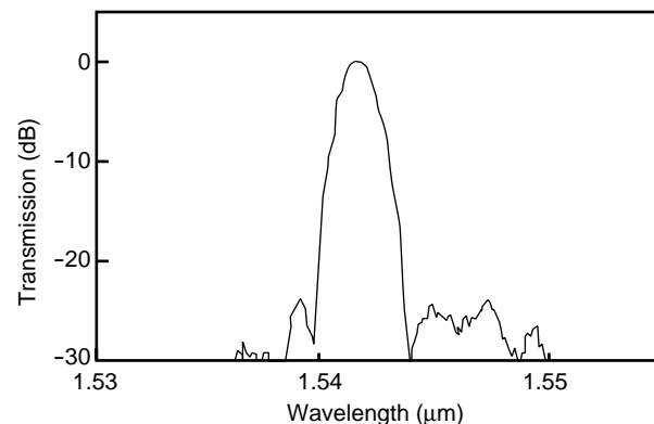
Figure 5 Transmission characteristic of intersecting SAWG.
