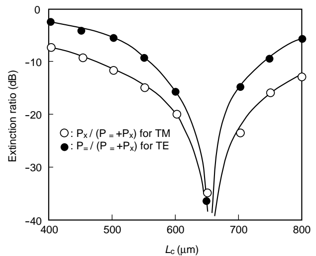
Figure 2 Characteristics of PBS.
