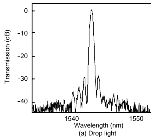
Figure 8 Integrated AOTF.
