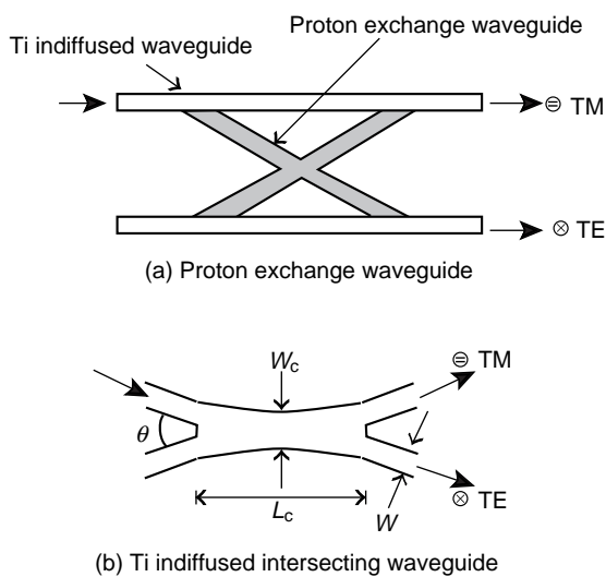
Figure 1 Waveguide PBS.
