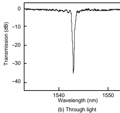
Figure 9 Filter characteristics.
