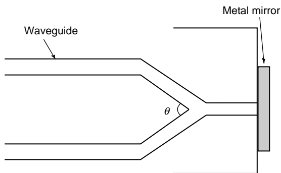
Figure 7 0-gap directional coupler type reflector.
