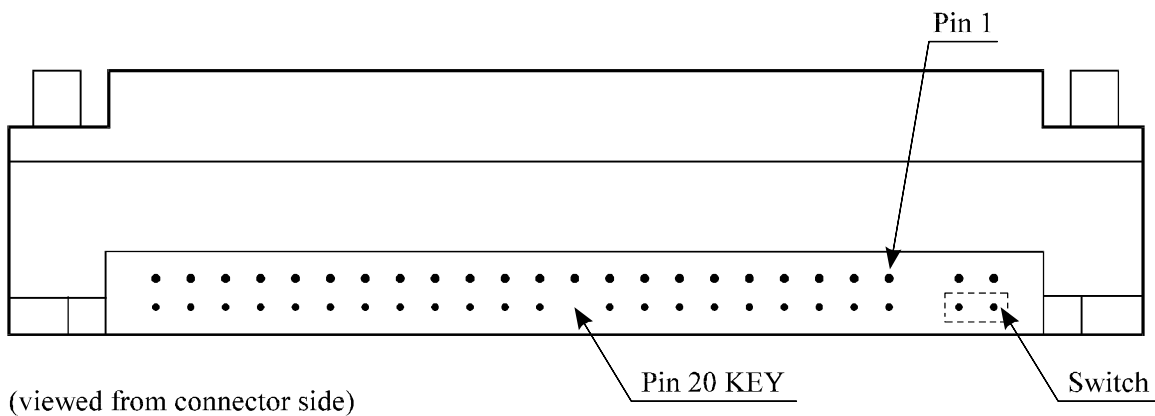
Figure 3.10 Jumper location
