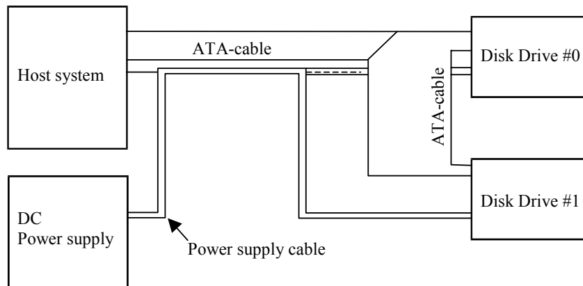
Figure 3.8 Cable connections
