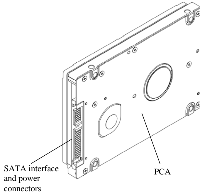
Figure 3.7 Connector locations
