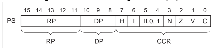
Figure 3.4-1 Structure of Program Status (PS)
