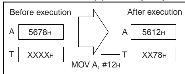
Figure 3.3-5 Operations between Accumulator (A) and Temporary Accumulator (T) (16-bit Operations)
